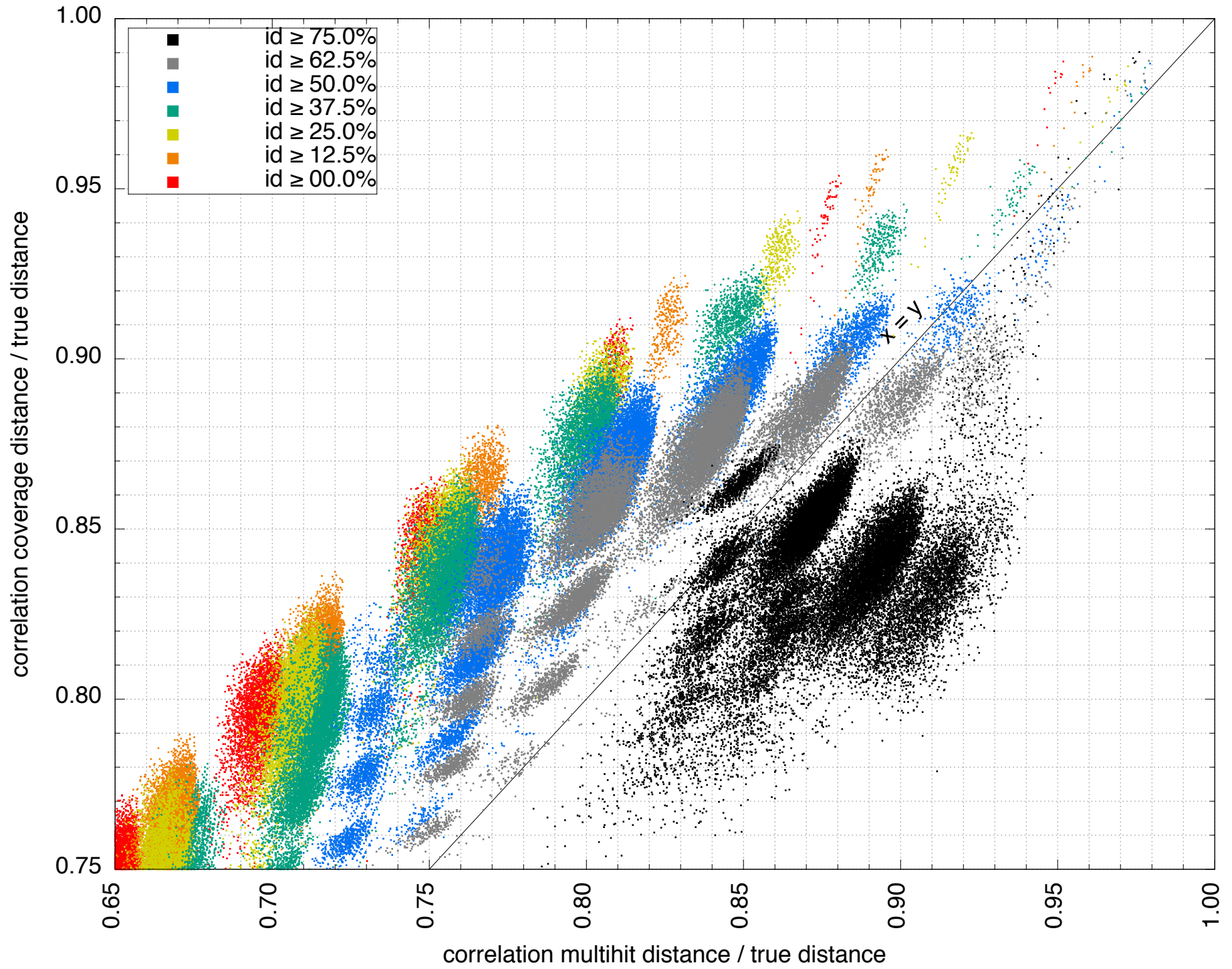
True distance Correlation with MultiHit (x) vs Coverage (y) distance
